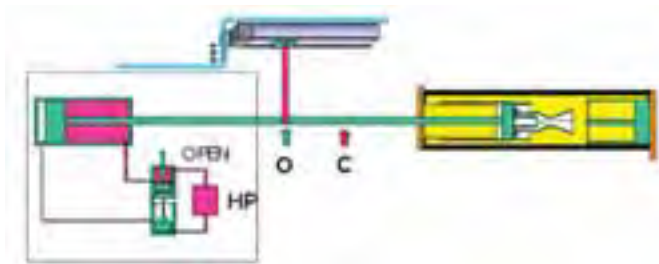
Linear transducer with breaker in open position
