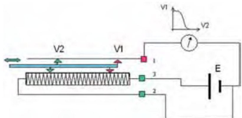
Fig. 2.12 Operation of a displacement transducer
