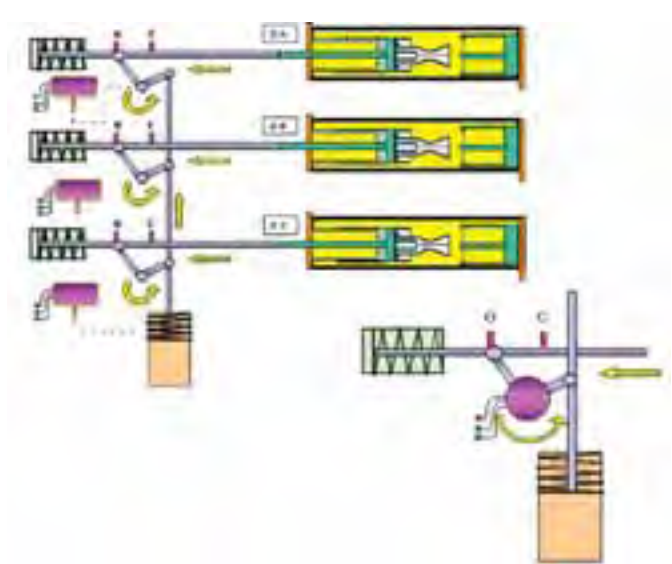
Fig. 2.3b Example using rotary transducers
