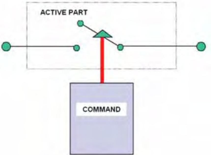
Fig. 2.21 Circuit breaker principle
