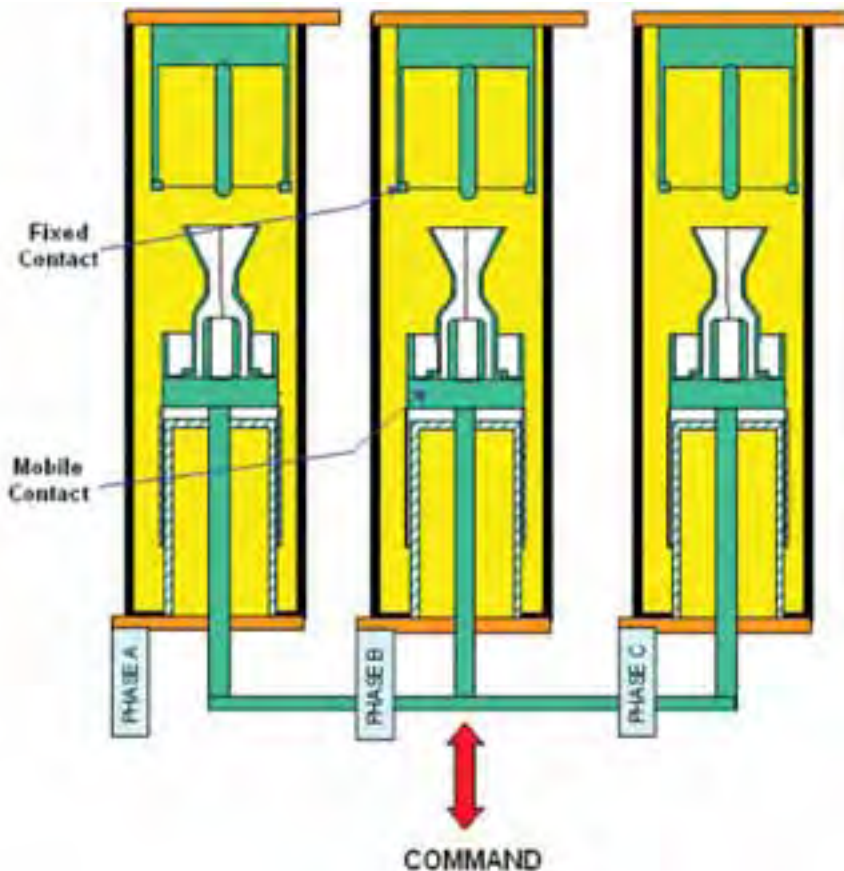
Fig 2.22 - Power section of the circuit breaker
