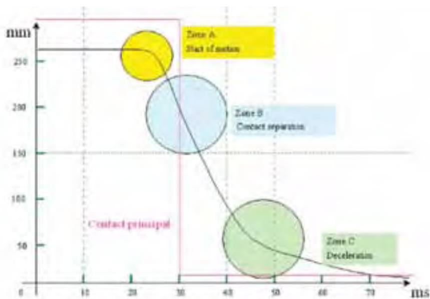
Fig 1.2 Displacement curve on Open operation
