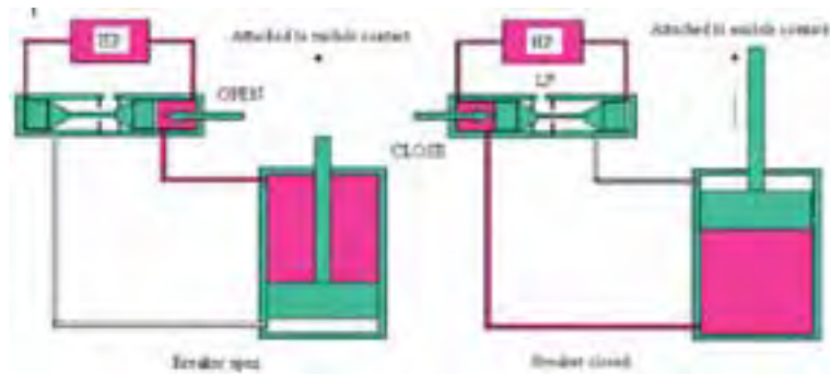
Fig 2.2.32 - Hydraulic command
