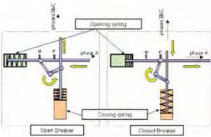
Fig 2.2.33 - Mechanical spring command
