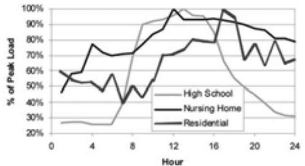
Figure 2 – Peak day load profiles.
