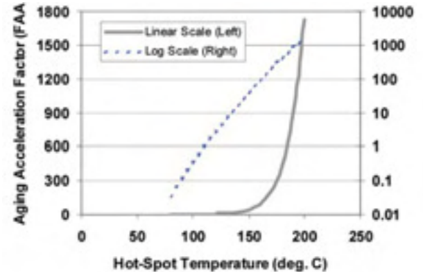
Figure 1 – Relationship between transformer insulation aging acceleration factor and winding hot-spot temperature.
