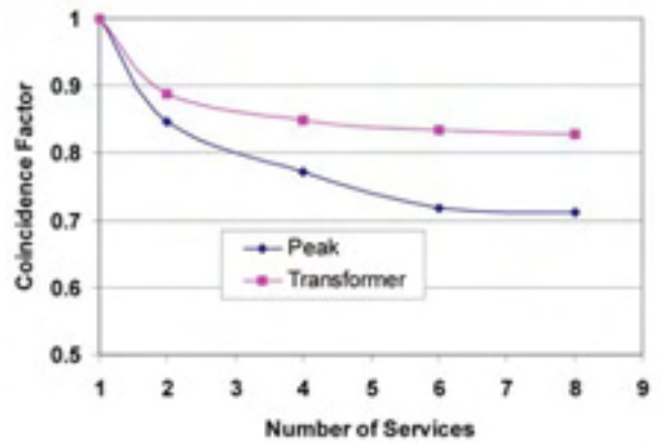
Figure 8 – Comparison of peak and transformer thermal coincidence factors for residential loads without electric space heat.
